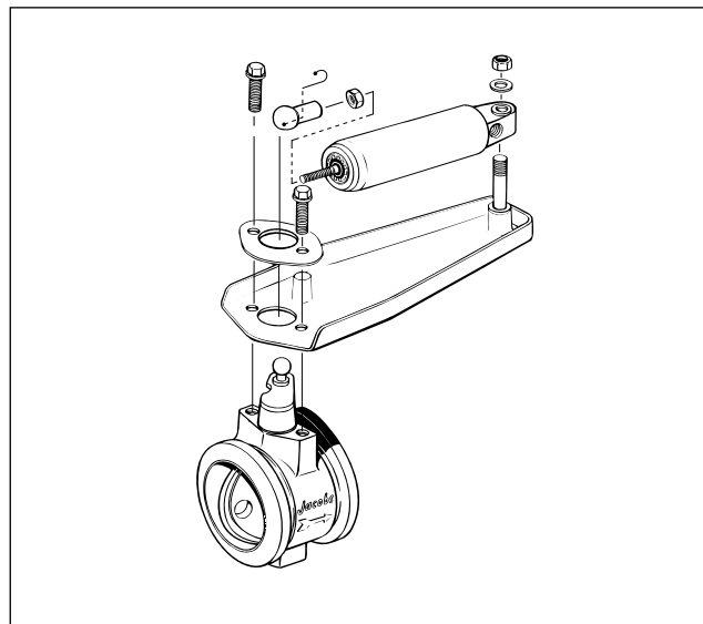
Exploded view of exhaust brake assembly
