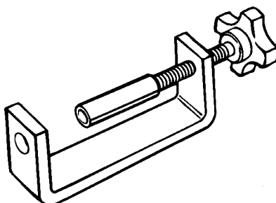
Slave Piston Removal Tool P/N 018238
